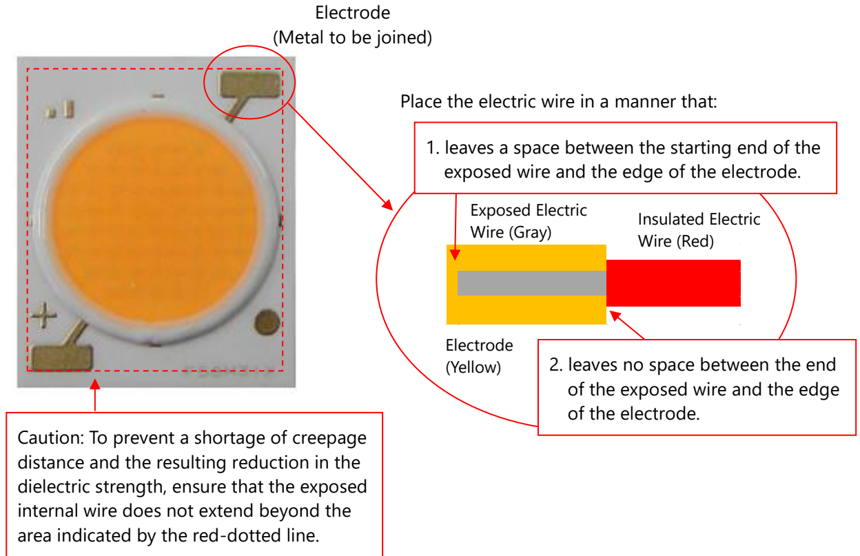
Figure 2. Schematic diagram of how to strip the wire
