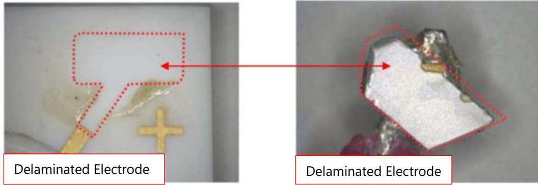
Figure 3. Electrode Delamination (Example of a Reported Failure)
