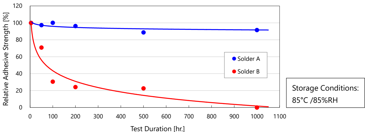
Figure 4. Reduction in the Adhesive Strength between the Electrode and Substrate over Time (Example)
